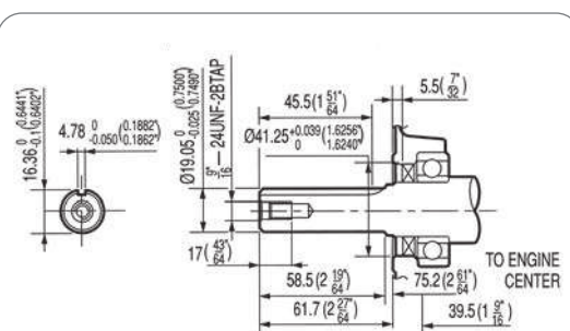
Albero - Shaft Mod.T/Q \varnothing 19,05 \text{ mm}
