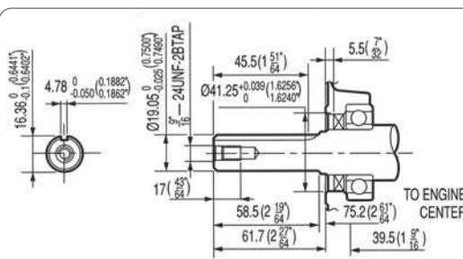
Albero - Shaft Mod.T/Q \varnothing 19,05 \text{ mm}
